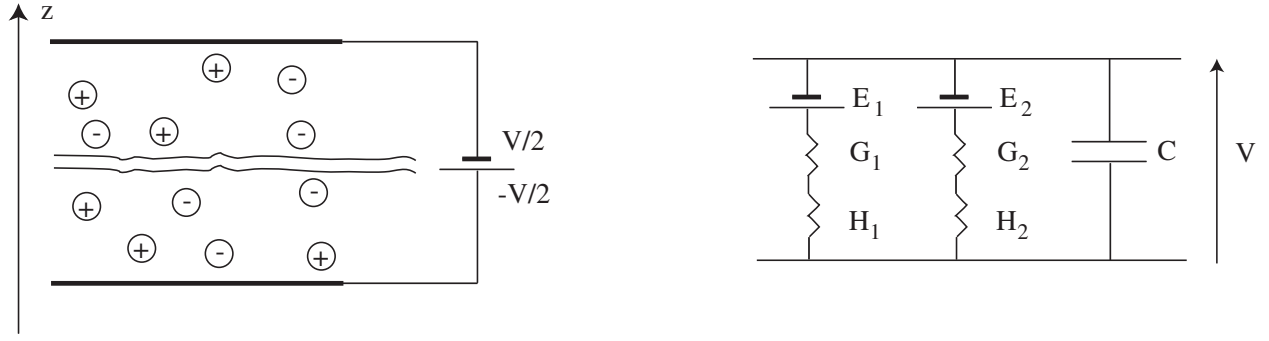
Fig. 1: Left: sketch of a quasi-planar fluid membrane embedded in an electrolyte in the presence of an applied potential difference and concentration gradients (not represented). Right: equivalent electrical circuit, with the contribution of the two ions k = 1, 2 in parallel, and for each ion, two conductances ( G_k for the membrane and H_k for the electrolyte) and an electromotive force E_k in series. When the finite thickness of the bilayer is included, there is also a capacitor C in parallel which contains contributions from Debye layers and from the membrane.
