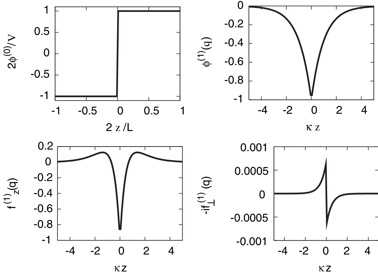
Fig. 2: Solutions of the electrokinetic equations for a membrane of zero thickness and symmetric ions concentrations n^- = n^+ = n . The parameters used in this figure are V = 50 mV, L = 1 \mu m, G_1 = G_2 = 10 \Omega^{-1}/\text{m}^2 , D_1 = D_2 = 10^{-5} \text{cm}^2/\text{s} and n = 16.6 mM. Top: left: normalized potential at zeroth order 2\phi^{(0)}(z)/V as a function of 2z/L . Right: normalized potential at first order in membrane undulation \phi^{(1)}(q, z) for a wave vector q = 10^6 \text{m}^{-1} , the normalization factor is h(q)\sigma 4\pi/\epsilon . Bottom: left: normalized force along z at first order f_z^{(1)}(q, z) . Right: normalized force along \mathbf{q} at first order -if_{\perp}^{(1)}(q, z) (where i is the imaginary number). This is for the same wave vector and the normalization factor for the forces is h(q)\sigma^{\frac{1}{2}}\kappa^2 4\pi/\epsilon .
